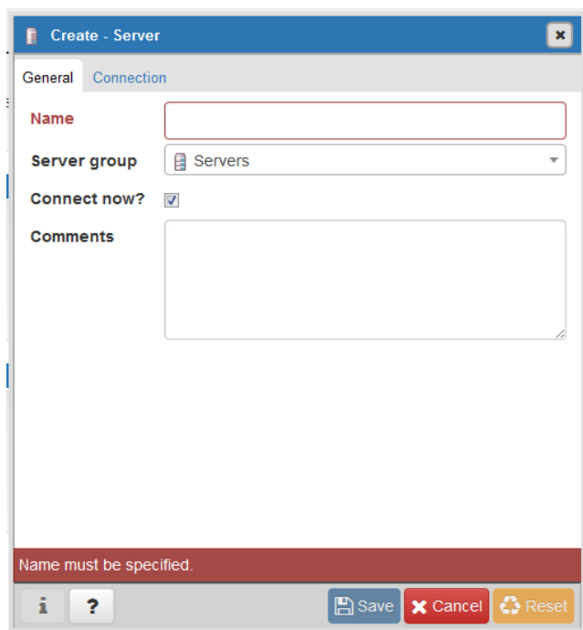
图6-2 General
